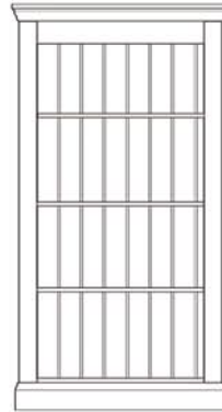
COL509 Bookcase H171xW96xD35 cm
